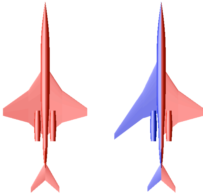
Maximum Range Design Baseline Maximum Range Design
