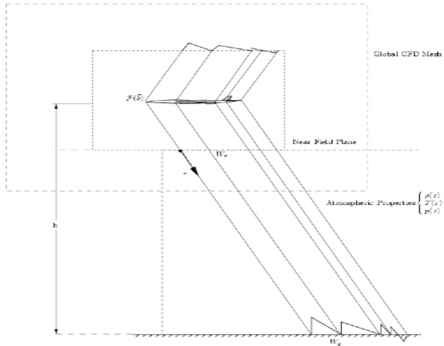
Figure 2: Sonic boom propagation procedure.
