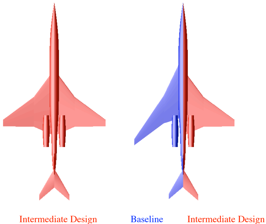
Figure 7. Result of Multi-Objective Optimization: Intermediate Design.
