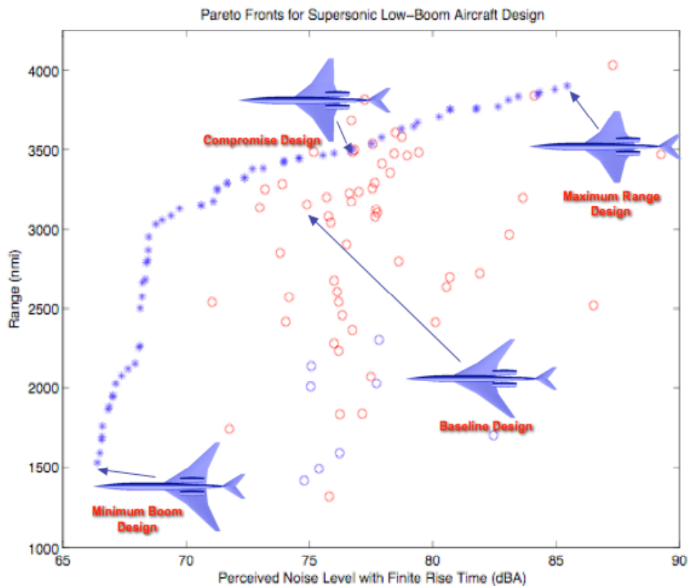
Figure 4. Results in Objective Space for the Multi-Objective Genetic Algorithm Optimization. Initial Population: open circles; Final Population: asterisks.
