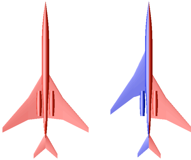
Actual Low-Boom Design Baseline Low-Boom Design
