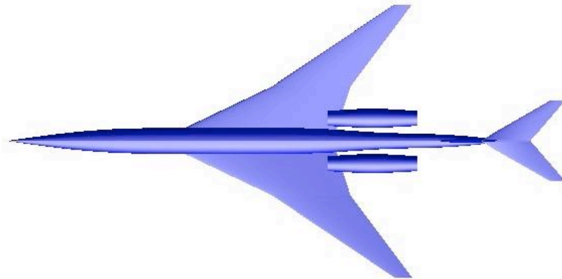
Figure 3. Top view of the baseline configuration for this design study.
